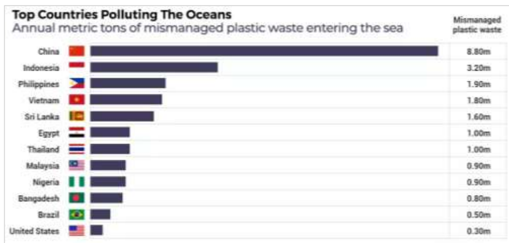
Fig. 2: Top countries Polluting the oceans. (2010)
